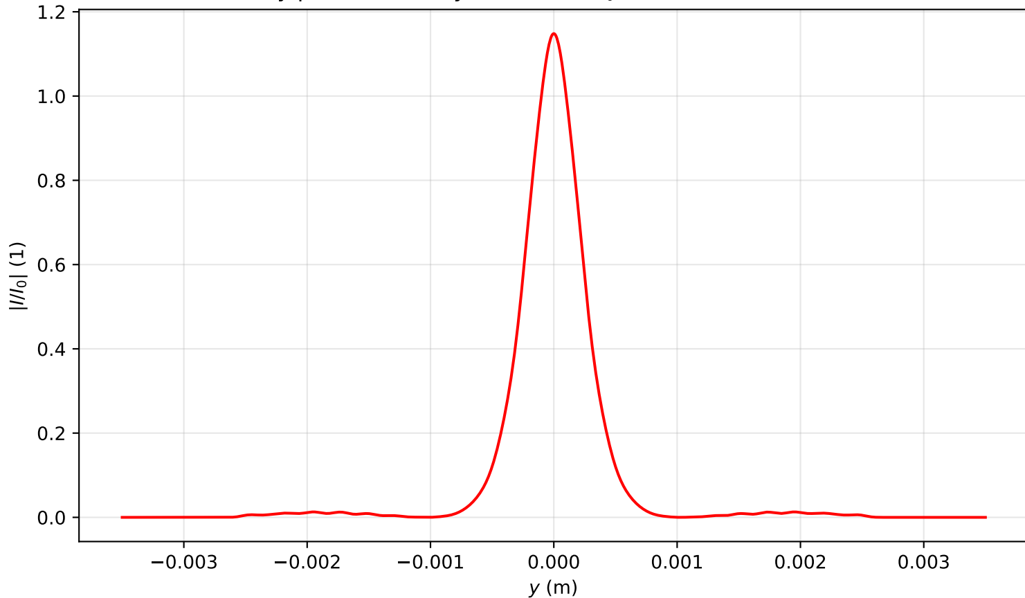
Intensity profile I(x=0, y, z=1.433)/I_0 , P_{in}=1.0P_{cr} , artificial time
